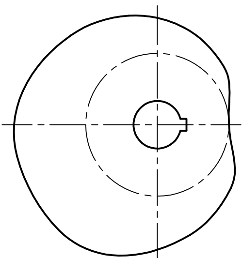
CAM PROFILE (FINISHED DRAWING)
