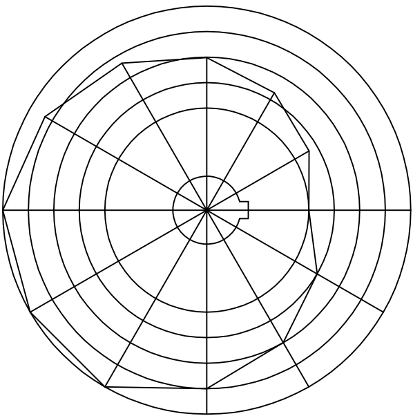
CAM PROFILE (CONSTRUCTION LAYOUT)
